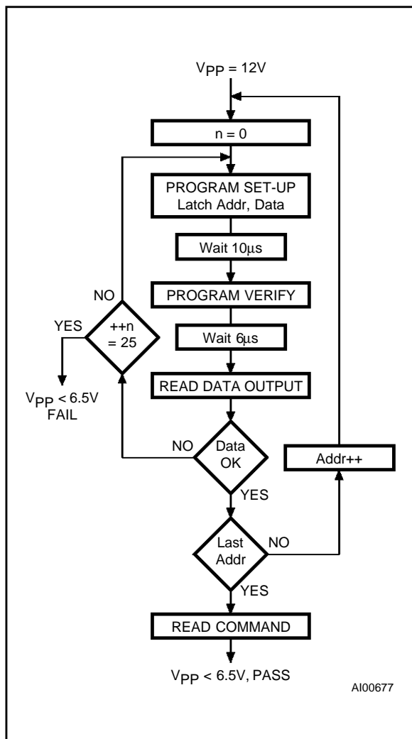
Figure 13. Programming Flowchart
